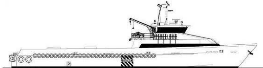
STBD PROFILE SCALE 1:120 REVISED 2006
