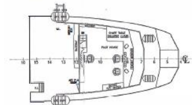
PILOT HOUSE DECK PLAN
