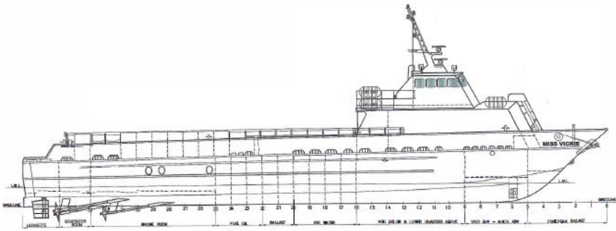
OUTBOARD PROFILE
